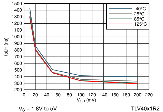
Figure 7-28. Propagation Delay Low-High vs Input Overdrive
