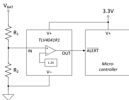
Figure 9-4. Under-Voltage Detection
