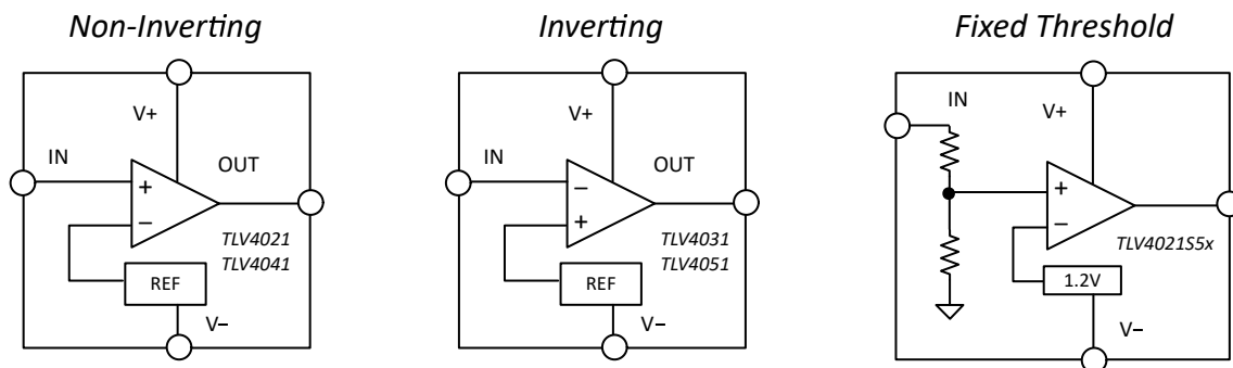
TLV40x1 Configurations
