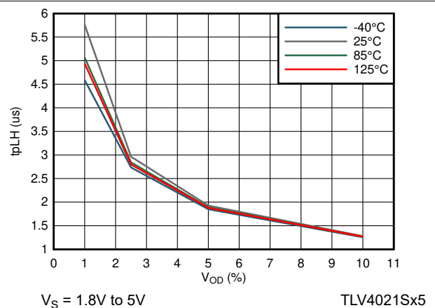
Figure 7-30. Propagation Delay Low-High vs Input Overdrive
