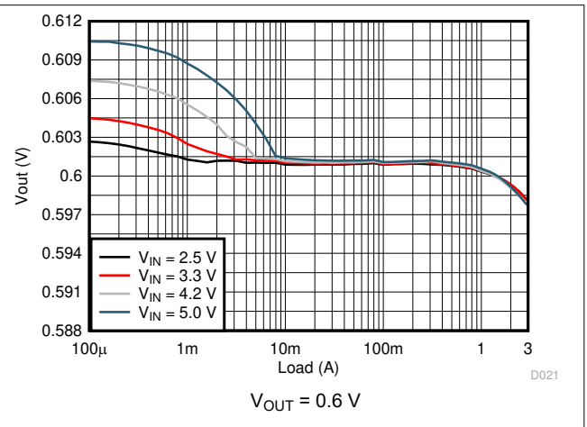
Figure 9-4. Load Regulation
