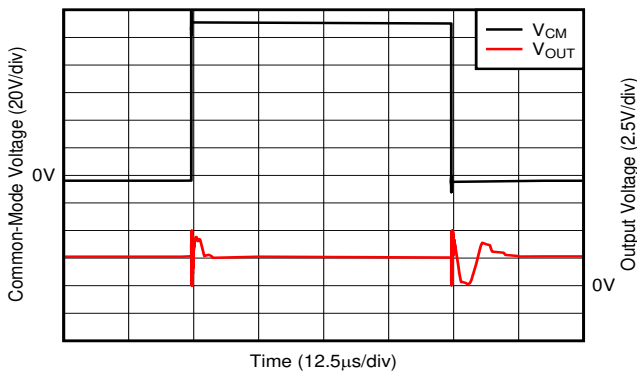
Figure 7-23. Common-Mode Voltage Fast Transient Pulse
