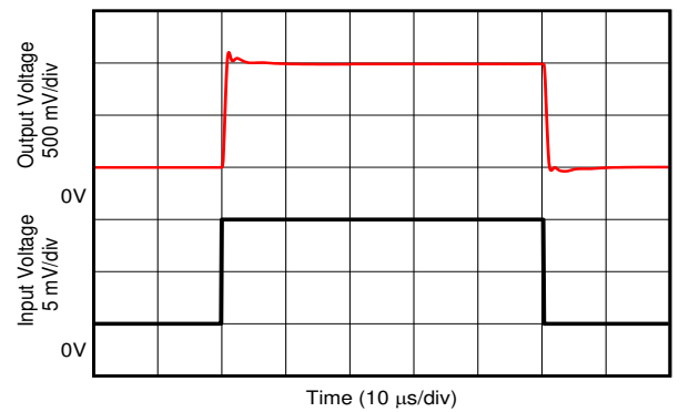
Figure 7-24. INA281x3 Step Response
