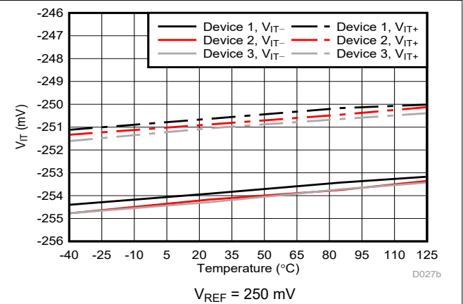
Figure 6-30. Cmp1 Trip Threshold vs Temperature
