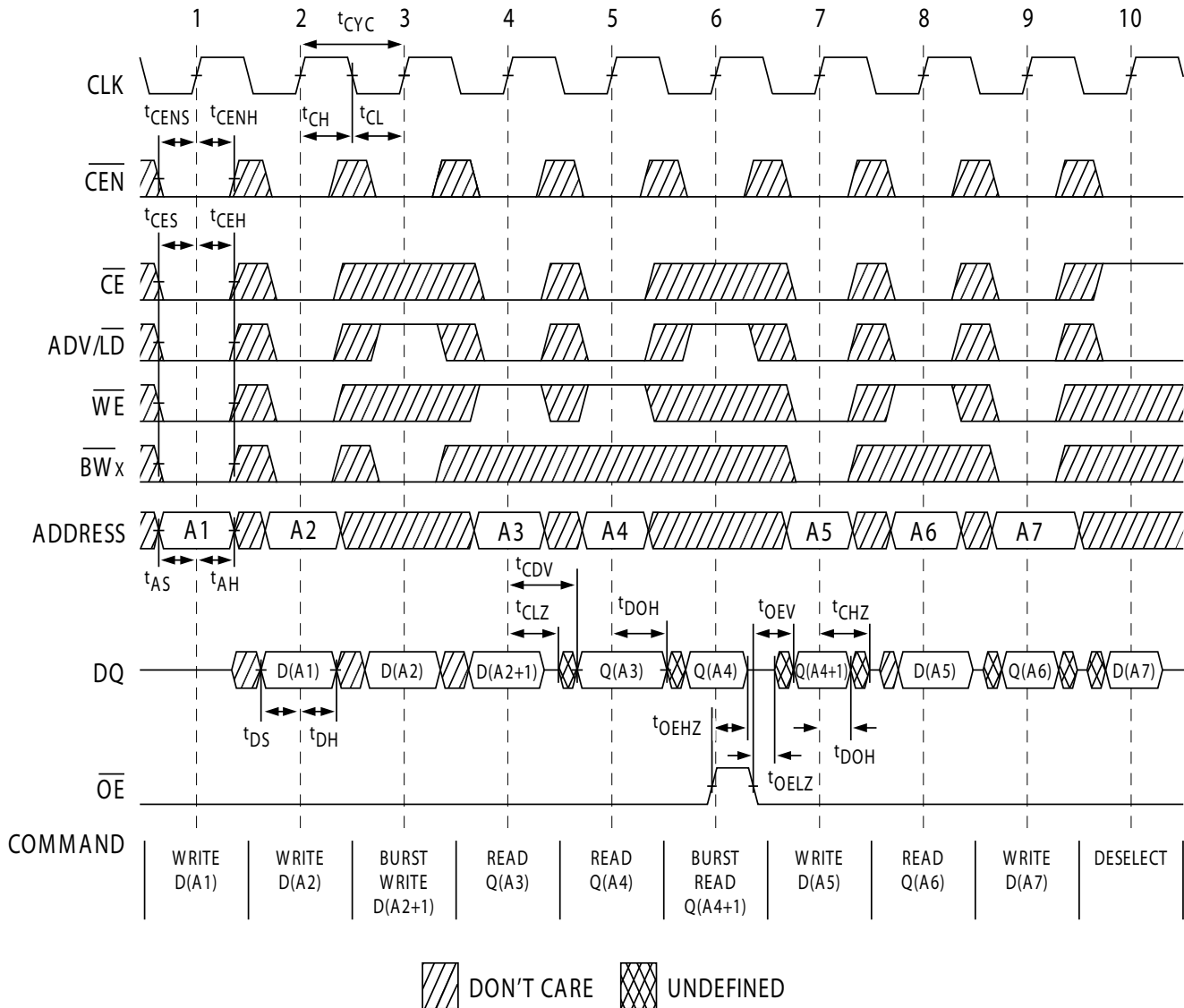
Figure 3. Read/Write Timing [21, 22, 23]
