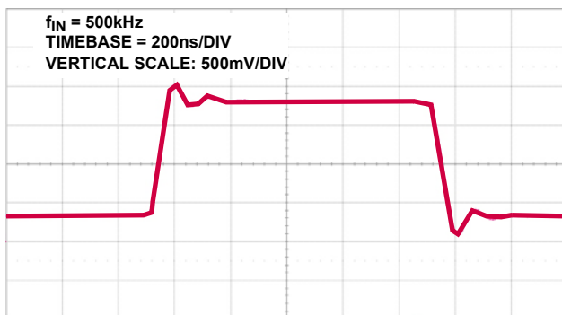
FIGURE 11. LARGE SIGNAL STEP RESPONSE
