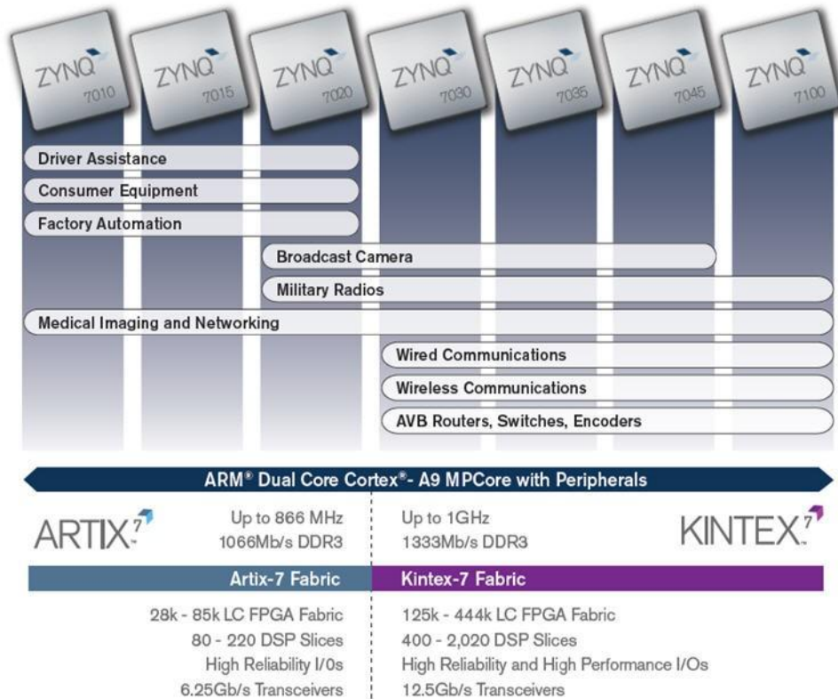
Zynq-7000 Devices
