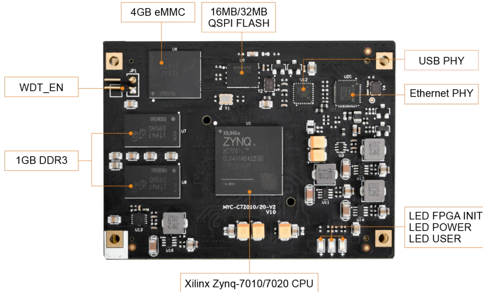
MYC-C7Z010/20-V2 CPU Module Top-view
