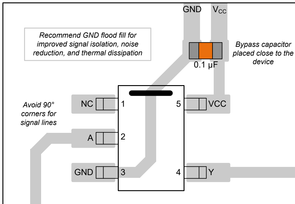
Figure 11-1. Example Layout for the SN74LV1T04-Q1
