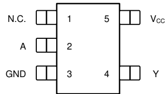
Figure 5-1. SN74LV1T04-Q1 DCK Package, 5-Pin SC70 (Top View)
