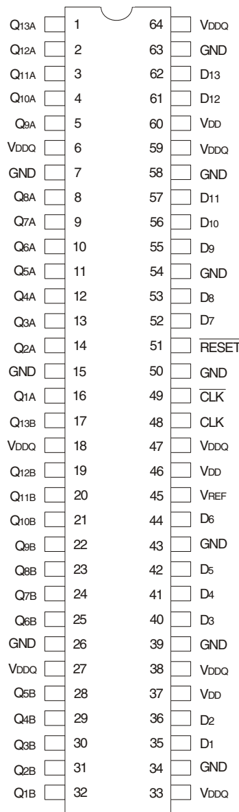
TSSOP TOP VIEW
