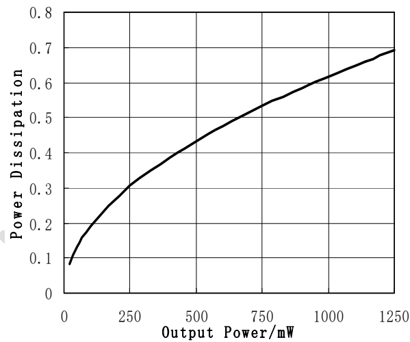
Figure 30 Power Dissipation vs. Output Power BTL mode, 5V, f=1 kHz, RL=80Ohm, THD+N<=1%
