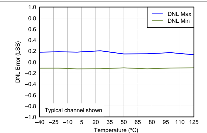
Figure 62. Differential Linearity Error vs Temperature
