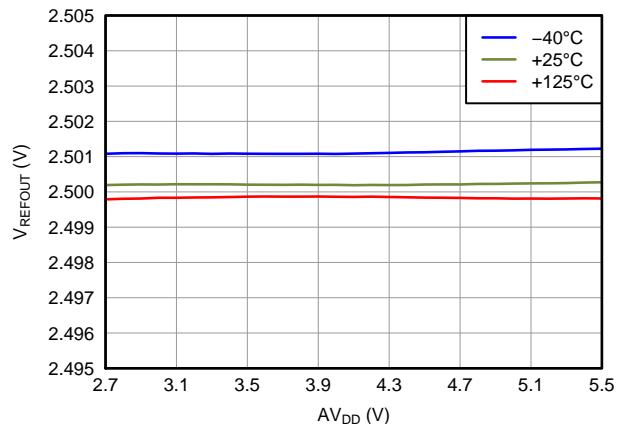
Figure 7. Internal Reference Voltage vs Supply Voltage
