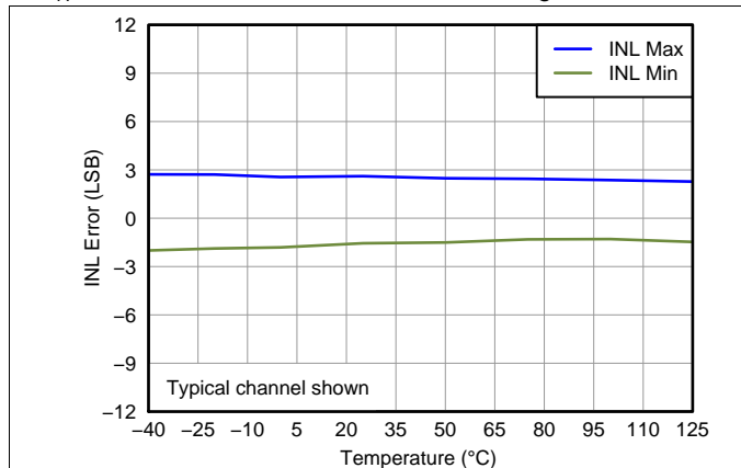
Figure 61. Linearity Error vs Temperature
