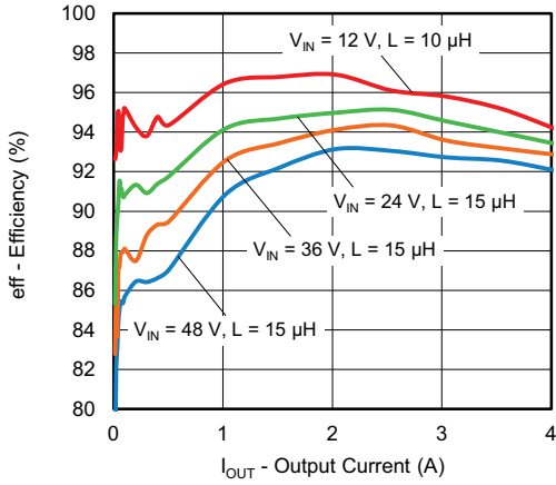
Fig. 22 - SiC468 Efficiency vs. Output Current, VOUT = 5 V
