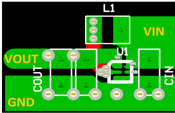
Figure 22. Layout Recommendation
