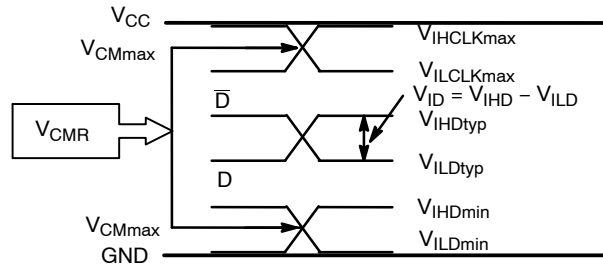
Figure 17. V_{CM} Diagram
