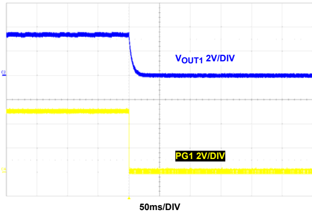
FIGURE 60. CH1 OTP
