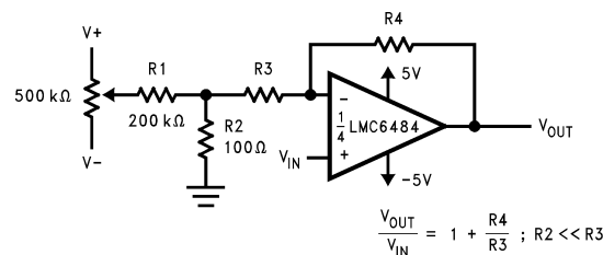
Figure 70. Non-Inverting Configuration Offset Voltage Adjustment
