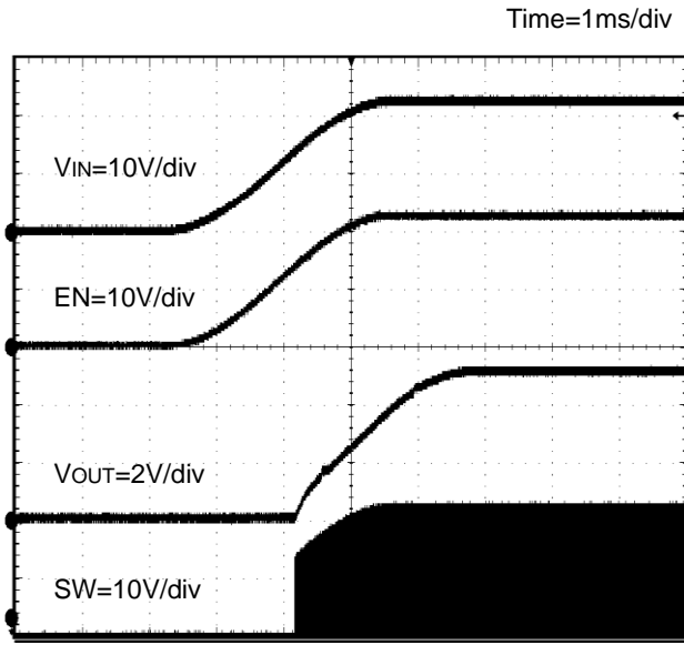
Figure 21. Power Up (V IN = EN) (V OUT = 5.0V)
