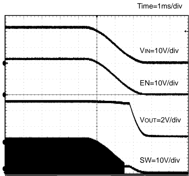
Figure 22. Power Down (V IN = EN) (V OUT = 5.0V)
