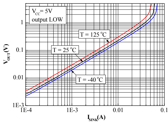
Figure 6. Output voltage vs. sinking current, output low, V CC = 5 V
