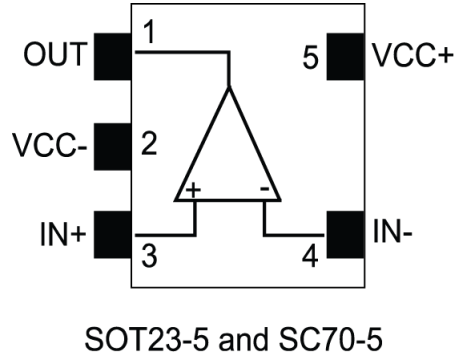
Figure 1. Pin configuration
