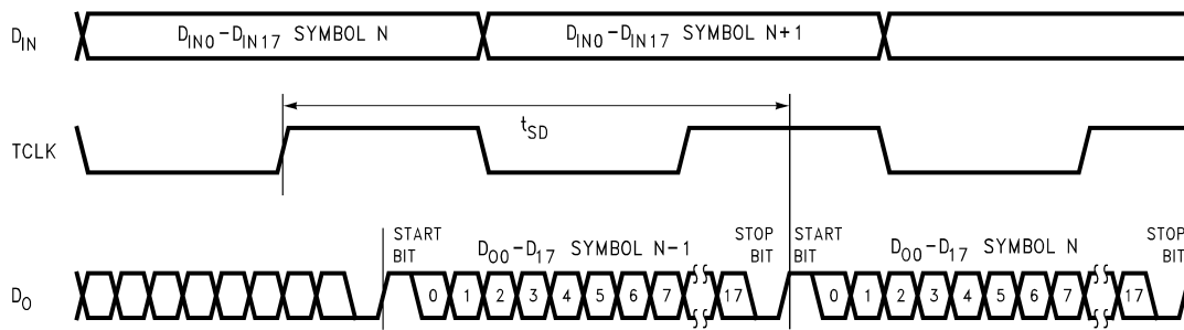
Figure 8. Serializer Delay
