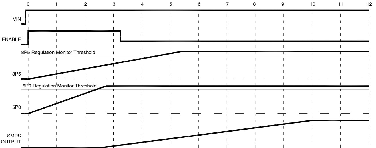
Figure 43. Enable High Time Long Enough to be Latched
