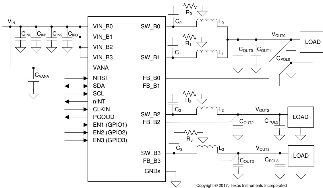
Figure 30. 2-Phase and Two 1-Phase Configuration (LP87523-Q1)
