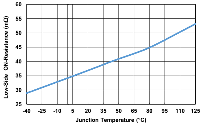
Figure 13. Low-Side rDS(ON) vs Junction Temperature
