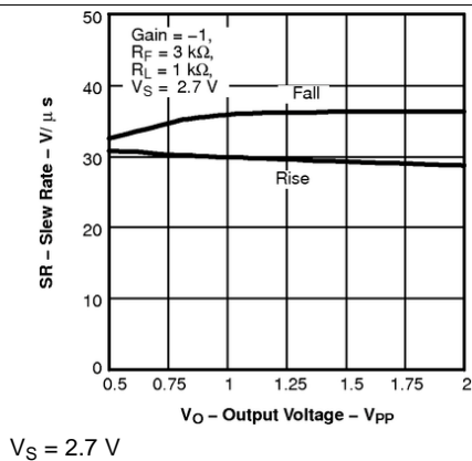
Figure 29. Slew Rate
