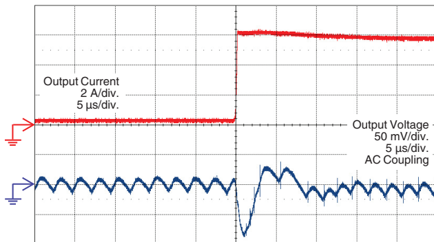
Transient Response in Continuous Conduction Mode (0.2 A to 6 A) (V_{IN} = 12\text{ V}, V_{OUT} = 1\text{ V}, f_{SW} = 500\text{ kHz})
