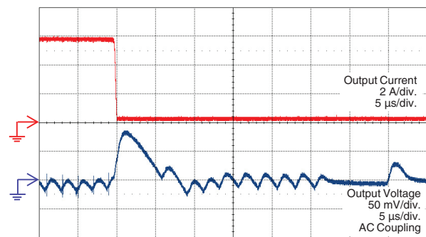
Transient Response in Power Save Mode (6 A to 0.2 A) (V_{IN} = 12\text{ V}, V_{OUT} = 1\text{ V}, f_{SW} = 500\text{ kHz at } 6\text{ A})
