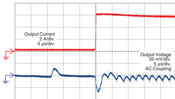
Transient Response in Power Save Mode (0.2 A to 6 A) (V_{IN} = 12\text{ V}, V_{OUT} = 1\text{ V}, f_{SW} = 500\text{ kHz at } 6\text{ A})
