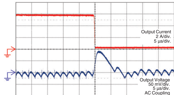
Transient Response in Continuous Conduction Mode (6 A to 0.2 A) (V_{IN} = 12\text{ V}, V_{OUT} = 1\text{ V}, f_{SW} = 500\text{ kHz})
