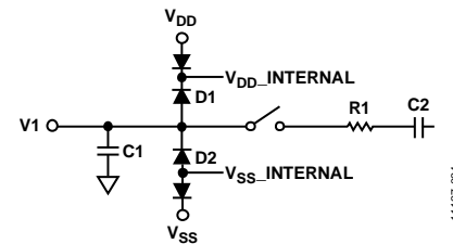
Figure 20. Equivalent Analog Input Structure
