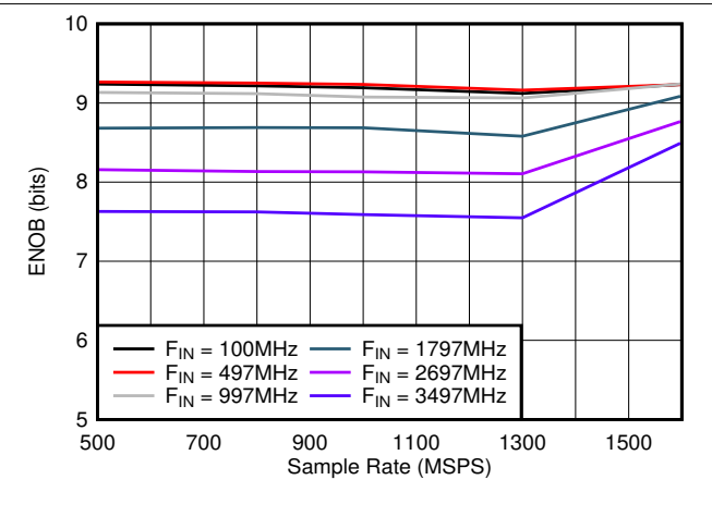
Figure 7-26. ENOB vs Sample Rate
