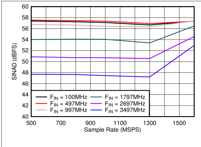
Figure 7-25. SINAD vs Sample Rate
