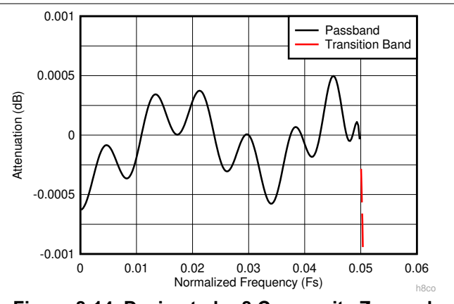
Figure 8-14. Decimate-by-8 Composite Zoomed Pass-Band Response
