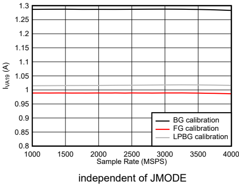
Figure 7-126. Dual Channel Mode: I_{VA19} vs Sample Rate
