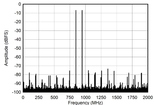
Figure 7-24. Dual Channel Mode: Two Tone FFT at 897 MHz
