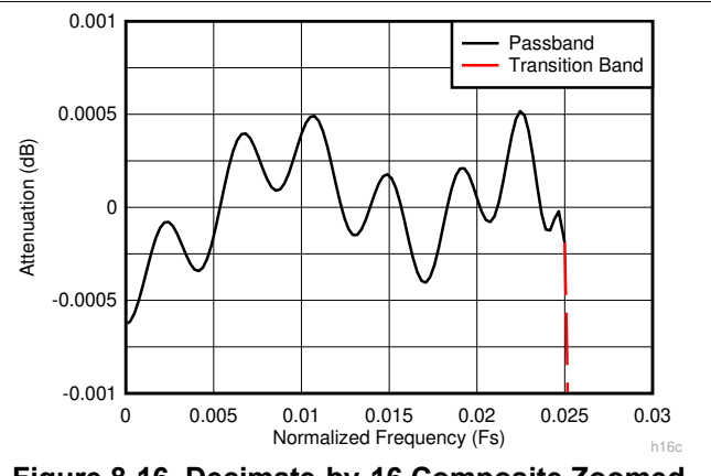
Figure 8-16. Decimate-by-16 Composite Zoomed Pass-Band Response
