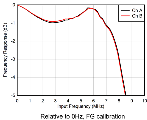
Figure 7-4. Input Response vs Input Frequency (zoomed)
