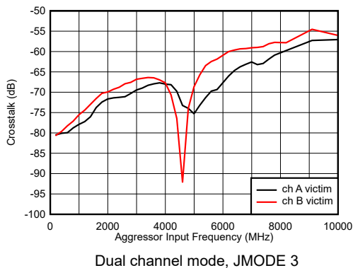
Figure 7-5. Crosstalk vs Input Frequency
