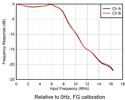
Figure 7-3. Dual Channel Mode: Input Amplitude vs Input Frequency
