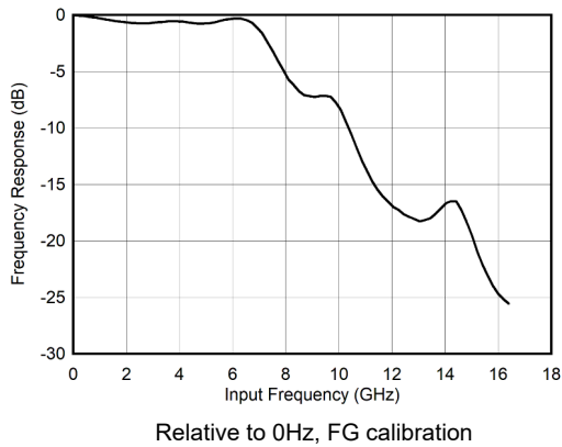
Figure 7-1. DES Mode: Input Amplitude vs Input Frequency
