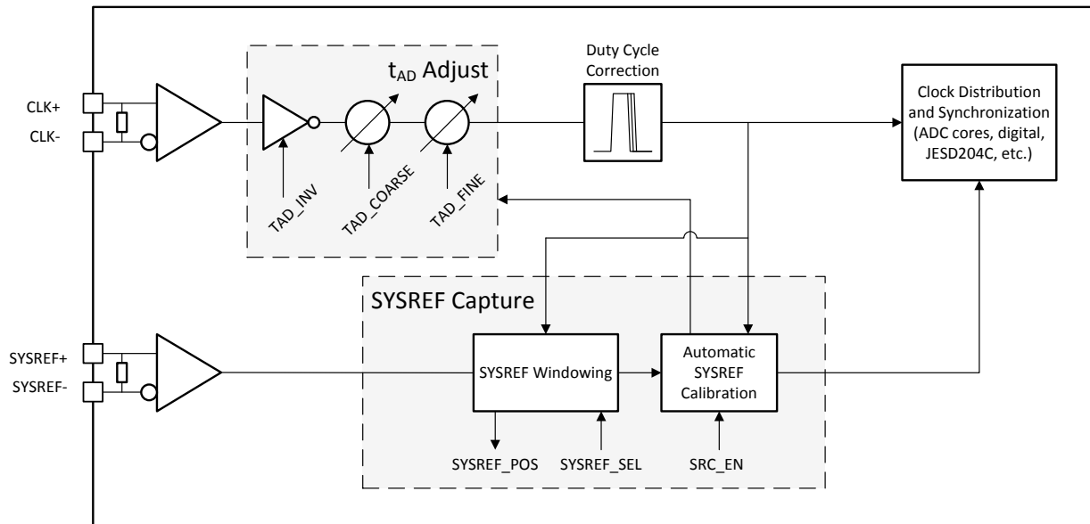
Figure 8-2. Clocking Subsystem
