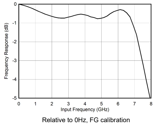
Figure 7-2. DES Mode: Input Response vs Input Frequency
