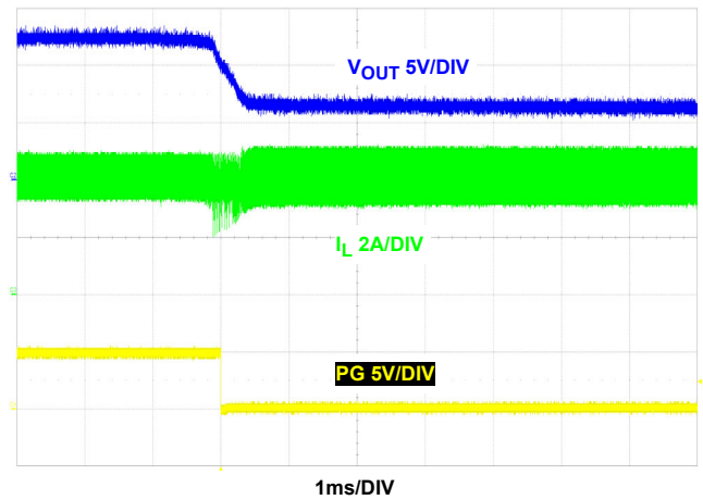
FIGURE 36. OVERCURRENT PROTECTION
