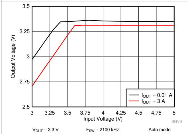
Figure 10-13. LM62440-Q1 Dropout Curve
