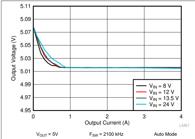
Figure 10-11. LM62440-Q1 Load and Line Regulation
