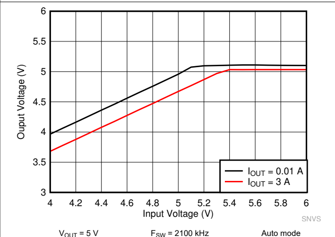
Figure 10-14. LM62440-Q1 Dropout Curve
