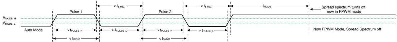
Figure 9-9. Spread Spectrum Disabled in Transition from Auto Mode to FPWM Mode
