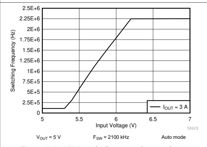
Figure 10-16. LM62440-Q1 Frequency Dropout Curve
