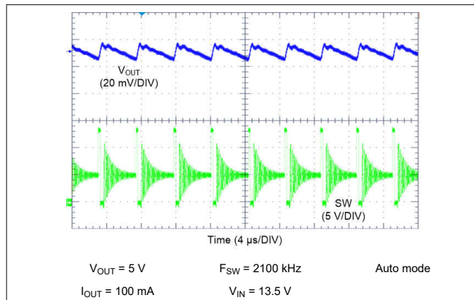
Figure 10-17. LM62440-Q1 Switching Waveform and V_{OUT} Ripple
