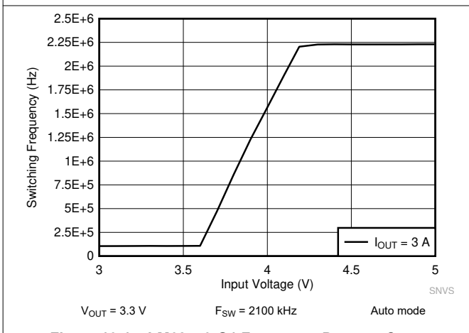
Figure 10-15. LM62440-Q1 Frequency Dropout Curve
