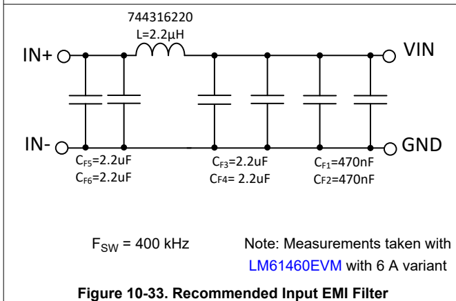
Figure 10-33. Recommended Input EMI Filter
