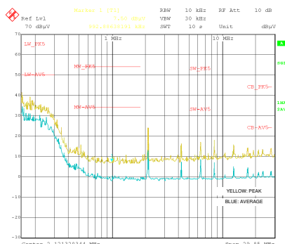
Conducted EMI: V_{\text{OUT}} = 5 \text{ V} , f_{\text{SW}} = 210 \text{ kHz}
