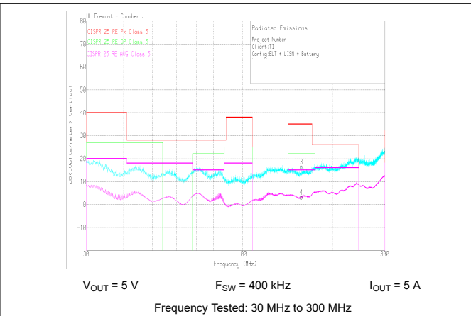
Figure 10-30. Radiated EMI Bicon Horizontal versus CISPR25 Limits, LM61460EVM
