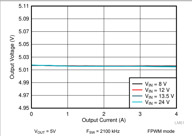
Figure 10-12. LM62440-Q1 Load and Line Regulation
