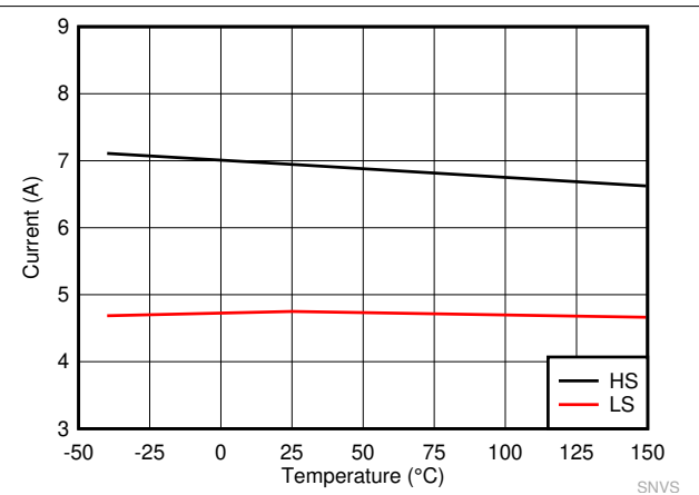
Figure 8-4. LM62440-Q1 High-Side and Low-Side Current Limits
