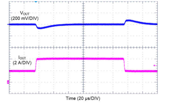
Figure 10-24. LM62440-Q1 Load Transient
