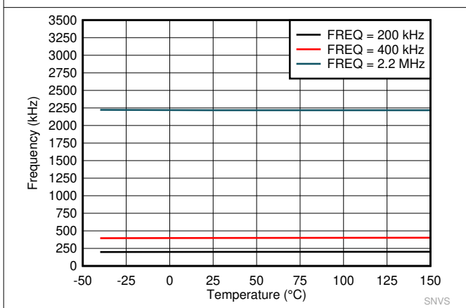
Figure 8-5. Switching Frequency Set by SYNC
