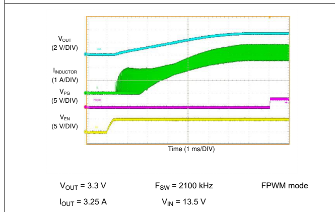
Figure 10-19. LM62440-Q1 Start-up with 3.25-A
