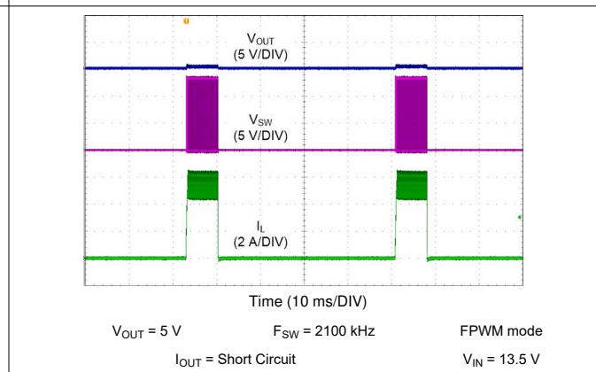
Figure 10-22. LM62440-Q1 Short Circuit Performance
