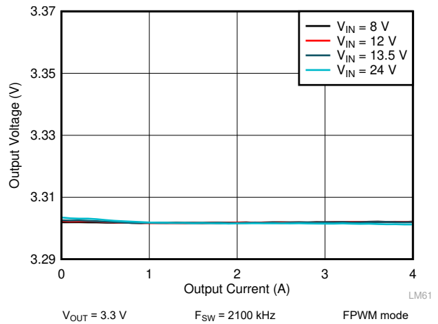
Figure 10-10. LM62440-Q1 Load and Line Regulation
