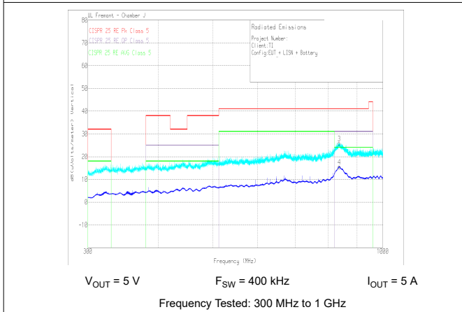
Figure 10-31. Radiated EMI Log Vertical versus CISPR25 Limits, LM61460EVM
