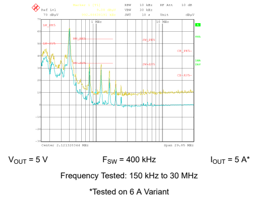
Figure 10-26. Conducted EMI versus CISPR25 Limits (Yellow: Peak Signal, Blue: Average Signal), LM61460EVM
