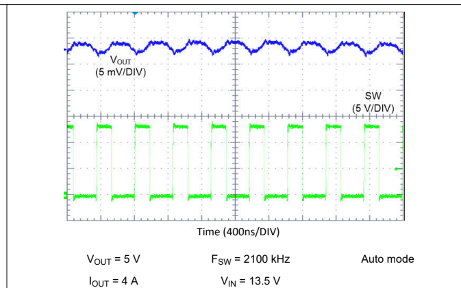
Figure 10-18. LM62440-Q1 Switching Waveform and V_{OUT} Ripple
