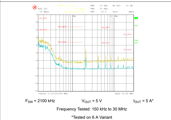
Figure 10-34. Conducted EMI versus CISPR25 Limits (Yellow: Peak Signal, Blue: Average Signal), LM61460EVM
