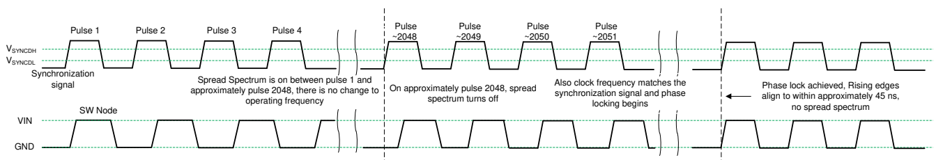
Figure 9-12. Synchronization Process
