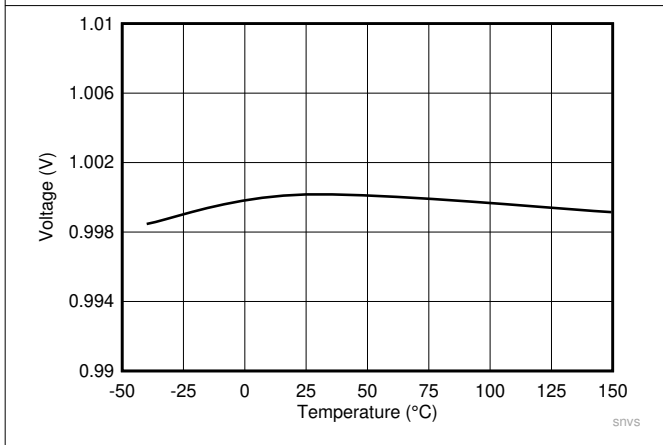
Figure 8-3. Feedback Voltage
