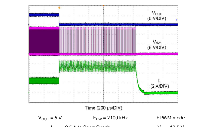
Figure 10-20. LM62440-Q1 Short Circuit Protection
