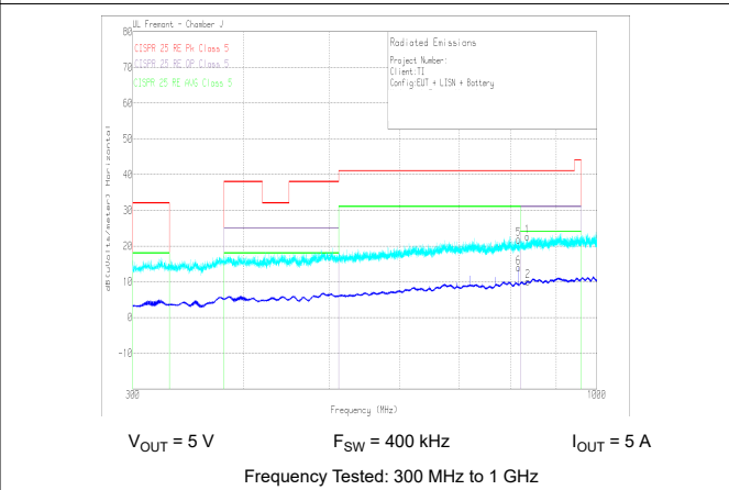
Figure 10-32. Radiated EMI Log Horizontal versus CISPR25 Limits, LM61460EVM
