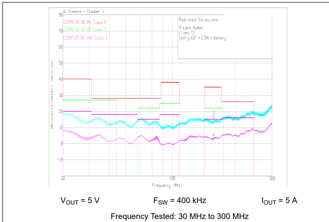
Figure 10-29. Radiated EMI Bicon Vertical versus CISPR25 Limits, LM61460EVM
