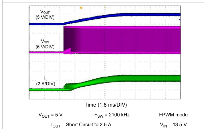
Figure 10-21. LM62440-Q1 Short Circuit Recovery
